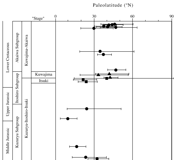
FIGURE 6. Variation of paleolatitudes of the Tetori Group. ▲: Kuwajima "Stage", ■: Itsuki "Stage".
