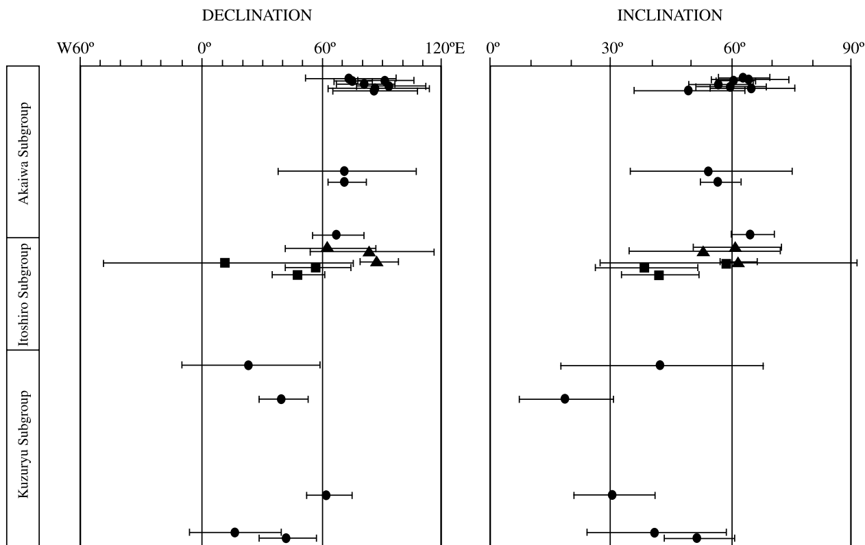
FIGURE 5. Temporal variations of mean declination and inclination at sampling sites. ▲: Kuwajima "Stage", ■: Itsuki "Stage".
